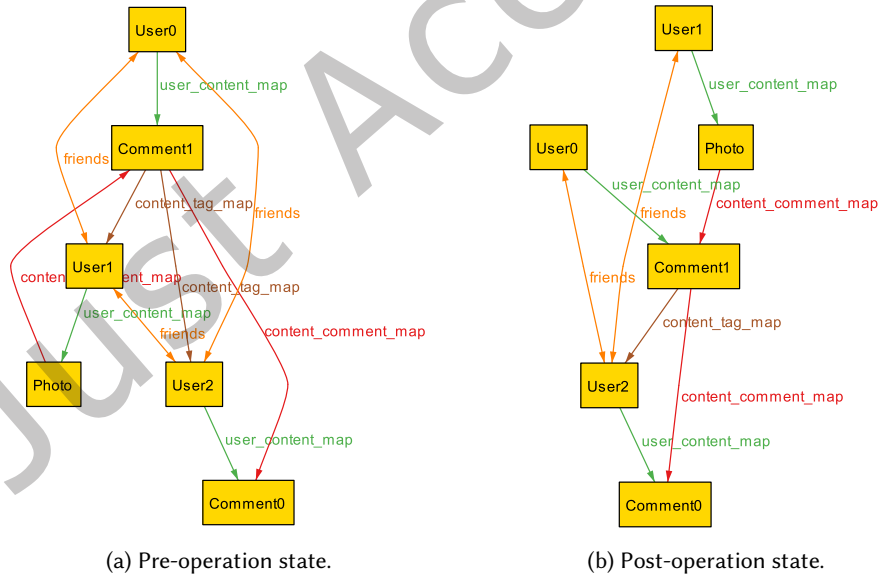
Fig. 3. Another example of inconsistency in Alloy-generated visualizations. The post-operation state (right) differs from the pre-operation state (left) only by the removal of two edges. Yet such a small semantic change propagates into a drastically different diagram.
