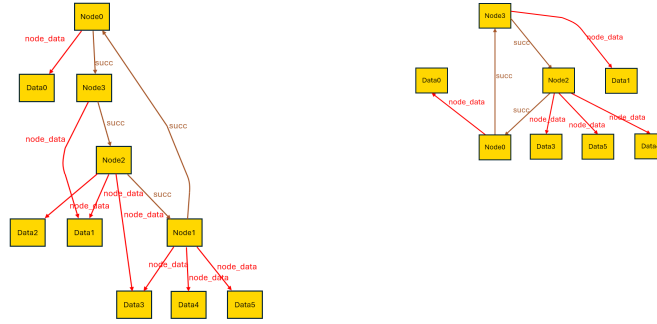
(a) A mockup of the Default Visualization , the Not-Consistent (NC) variant. Observe that the position of every node in the diagram has drastically changed.
